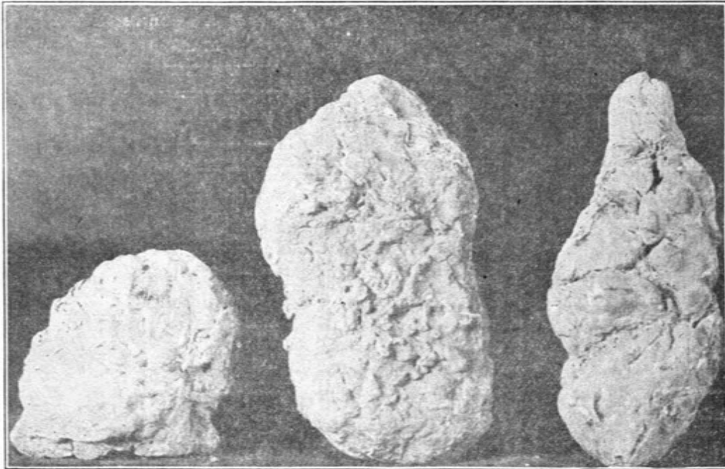
Fig 4. Phosphate Nodule NE. of SE \frac{1}{4} Sec. 33 T. 4 S., R. 9 W. 1 mile N. of Extreme SE. Corner of Cotton County, Oklahoma. Natural Size. A. C. Shead.
